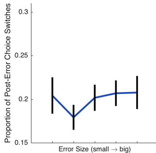
Fig. S2. Visual error size and choice behavior in experiment 1. For the Spatial condition of experiment 1, we examined whether the size of the visual error, the distance between the cursor and the target, affected choice behavior. To this end, we analyzed the miss trials that led to target choice switches, dividing them, for each participant, into five equally spaced bins based on the size of the observed visual cursor error ( \mu error \approx 0.35 cm). An ANOVA revealed that the size of the visual feedback error on miss trials did not influence the likelihood that the participant would change their target preference after such trials [ F_{(4,95)} = 0.49 , P = 0.75 ].
